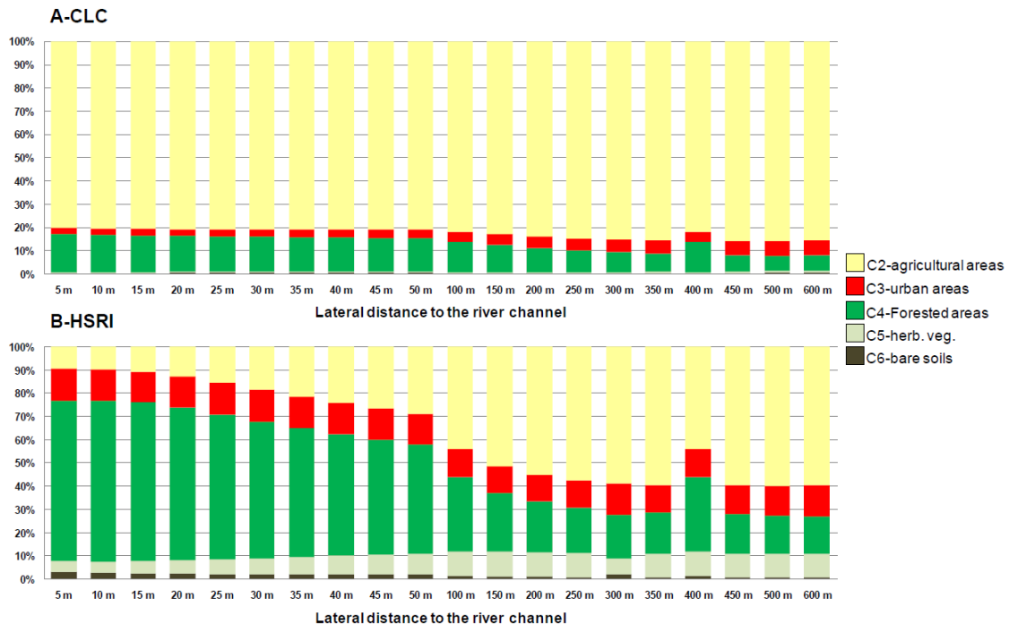
Figure 3. Variation of the area percentage of a given land cover type according to the lateral distance to the river channel on the Herault river reach. (A) from CORINE Land Cover (CLC) database, (B) from the High Spatial Resolution Imagery (HSRI)-derived map
