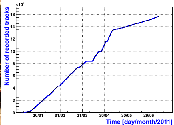
Figure 1. a) The detection setup at the Puy de Dôme. From left to right: (remote-)control station, HV supply and gas distribution system, GRPC detector and acquisition PC. b) Number of recorded muon tracks from January to July 2011 with three different detector configurations.
