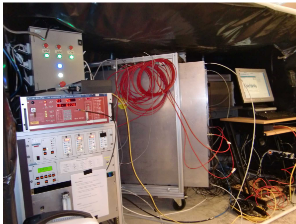
Figure 1. a) The detection setup at the Puy de Dôme. From left to right: (remote-)control station, HV supply and gas distribution system, GRPC detector and acquisition PC. b) Number of recorded muon tracks from January to July 2011 with three different detector configurations.
