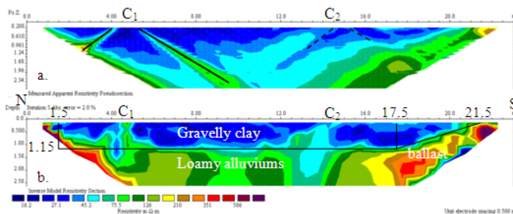
Figure 2. ERT 1 intersects the two cracks C_1 and C_2 . a. Measured apparent resistivity pseudosection (dipole-dipole array). b. Inverse model resistivity section (robust inversion).
