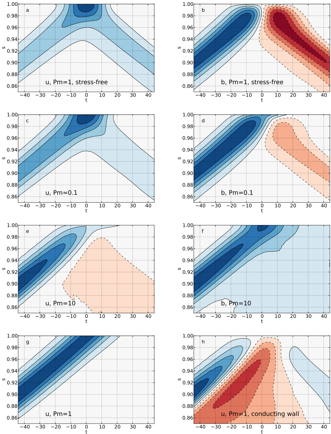
FIG. 4. Space-time diagrams of the reflection of a TAW for S \simeq 10^4 and \ell = 0.02 recorded in the equatorial plane, near the equator. Top line : stress-free boundary with Pm = 1 ( R = 0.88 ), (a) the azimuthal angular velocity u_\phi/s and (b) the azimuthal magnetic field b_\phi (changing sign). Second line : No-slip boundary with Pm = 0.1 ( R = 0.40 ), (c) the azimuthal angular velocity u_\phi/s and (d) the azimuthal magnetic field b_\phi (changing sign). Third line : No-slip boundary with Pm = 10 ( R = -0.17 ), (e) the azimuthal angular velocity u_\phi/s (changing sign) and (f) the azimuthal magnetic field b_\phi . Bottom line : azimuthal angular velocity u_\phi/s for no-slip boundary with Pm = 1 showing no reflection ( R = 0 ) for insulating boundary (g), and little reflection when the insulator is replaced by a solid conductive layer (h).
