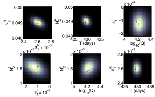
Fig. 4. Joint probability density functions of x , T_{FCN} , s_1 and N_2 estimated from the nutation amplitudes.
