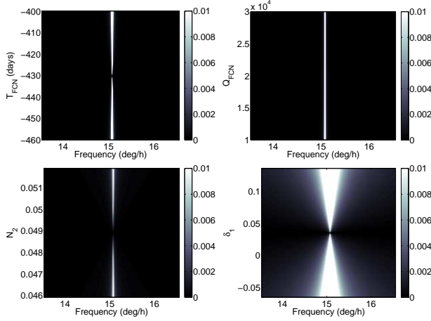
Fig. 1. Sensitivity of the gravimetric transfer function T^{(g)} to the parameters T_{FCN} , Q_{FCN} , N_2 , and \bar{\delta}_1^R .
