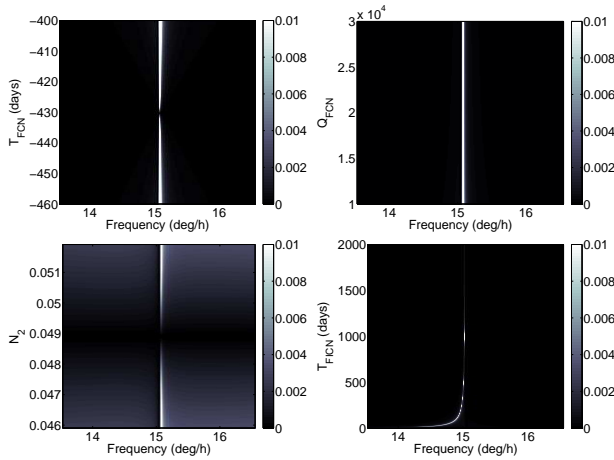
Fig. 2. Sensitivity of the nutation transfer function T^{(n)} to the parameters T_{FCN} , Q_{FCN} , N_2 , and T_{FICN} .
