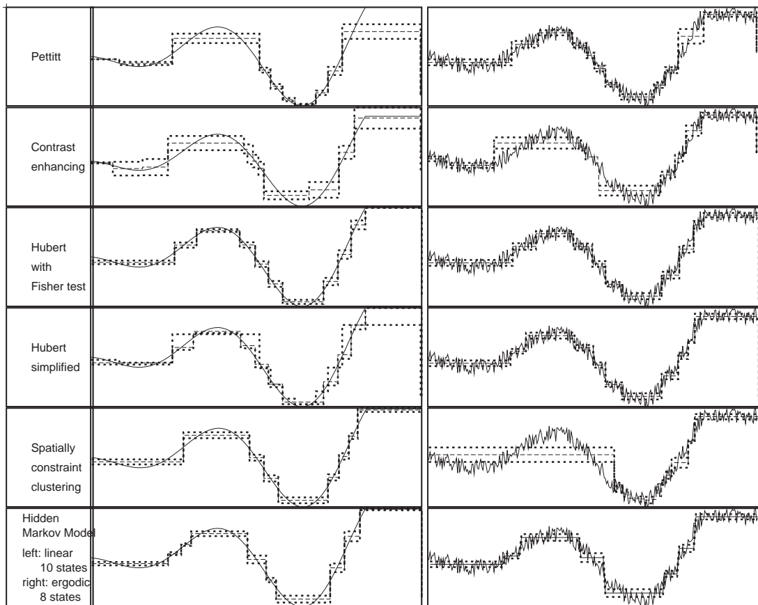
Figure 12: 3 rd template. Left without noise; right: with noise.
