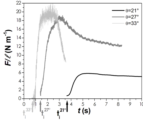
FIG. 4: Laboratory tests. Force per unit width, F/\ell , measured on the wall versus time t for three slope inclinations: \theta = 21^\circ (black color), 27^\circ (gray) and 33^\circ (light gray).
