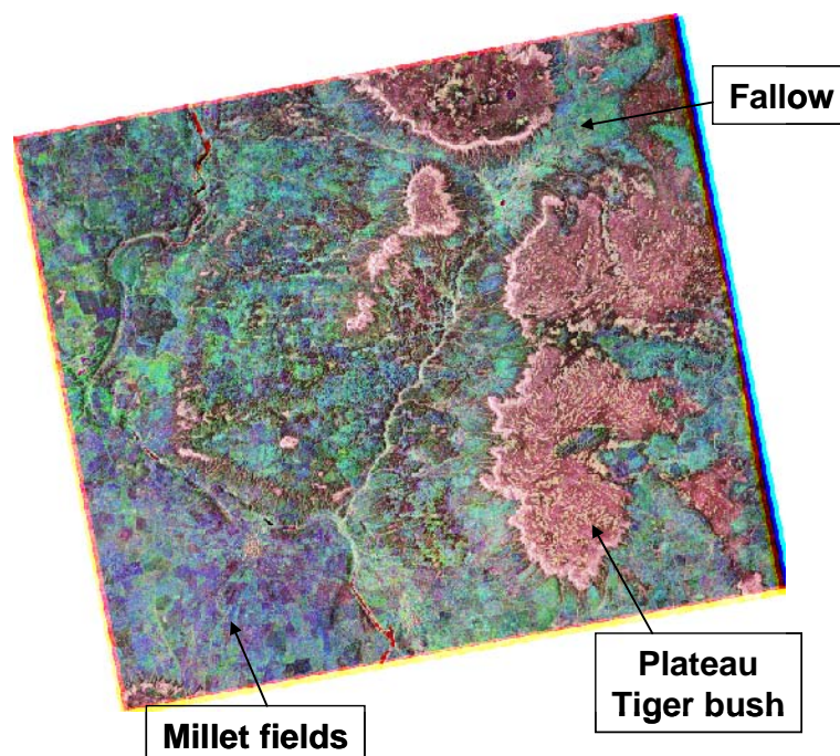
Banizoumbou, RGB= 29 May, 14 August and 08 October 2009
