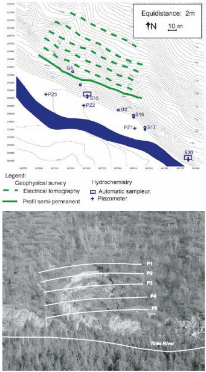
Fig. 4 Location of the five electrical profiles on the Clapiere landslide.
