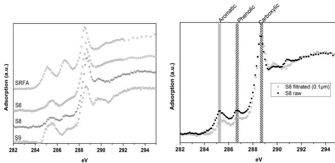
Fig. 2. On the left, a comparison between XANES spectra for the S6, S8 and S9 leachates (0.1 \mu\text{m} filter material) and for Suwannee river fulvic acid (left). On the right, the effect of the filtration on the recorded XANES spectra has been checked on the sample S8 by measuring both the non-filtered and the below 0.1 \mu\text{m} fractions.
