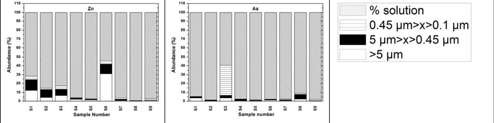
Fig. 1. Proportion of the different metals as a function of filter cut off.
