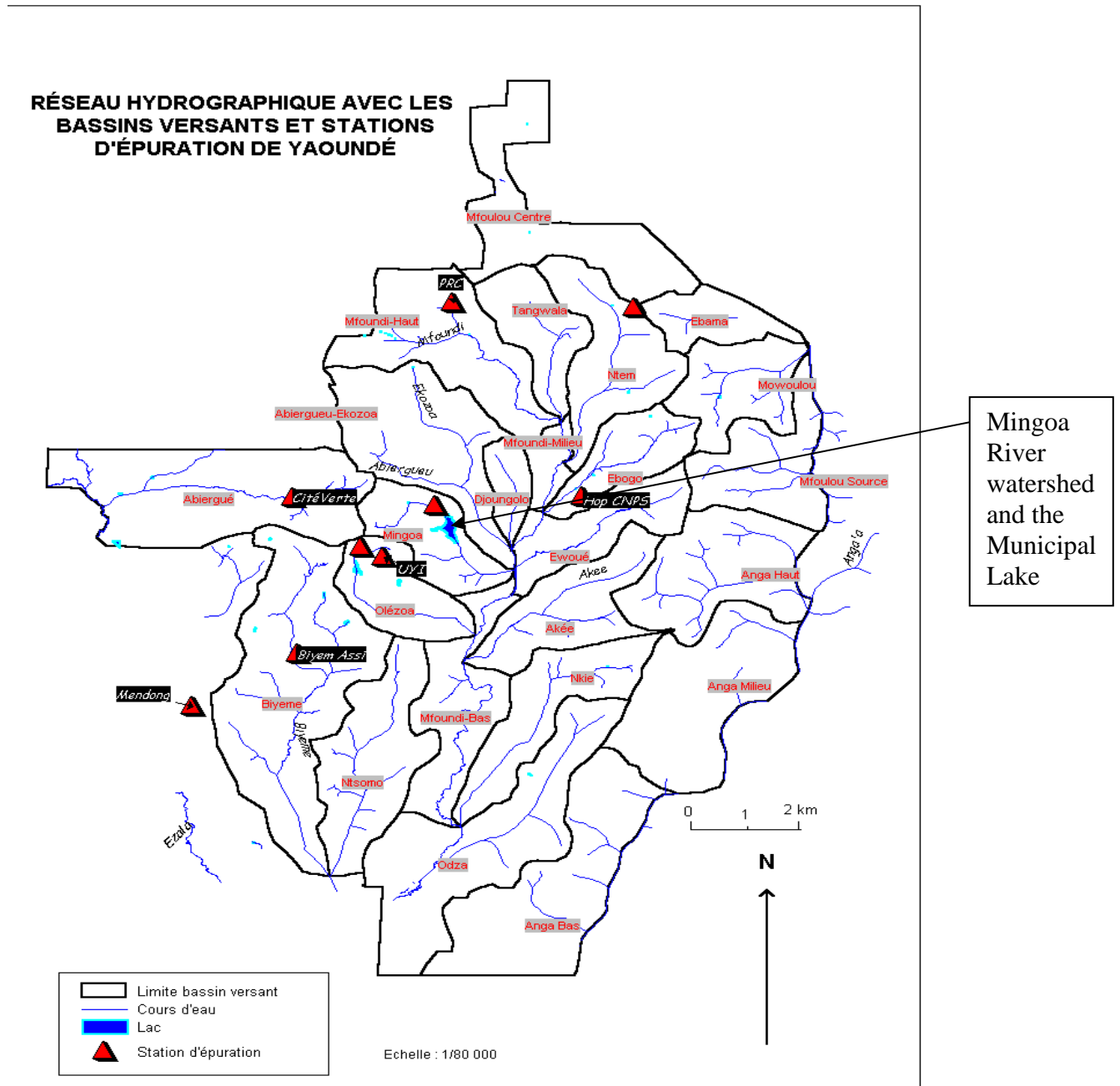
Figure 2: Water system of Yaoundé (LESEAU, 2007)
