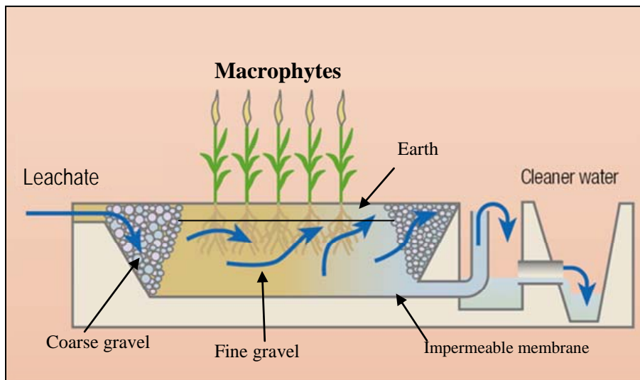
Figure 1: Main features of a sub-surface constructed wetland (SSCW)
