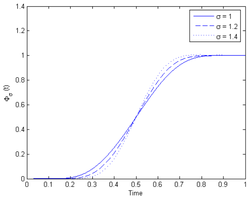
Figure 3: Dimensionless bump function. The bump function \phi_\sigma(t) is a Gevrey function of order 1 + 1/\sigma .
