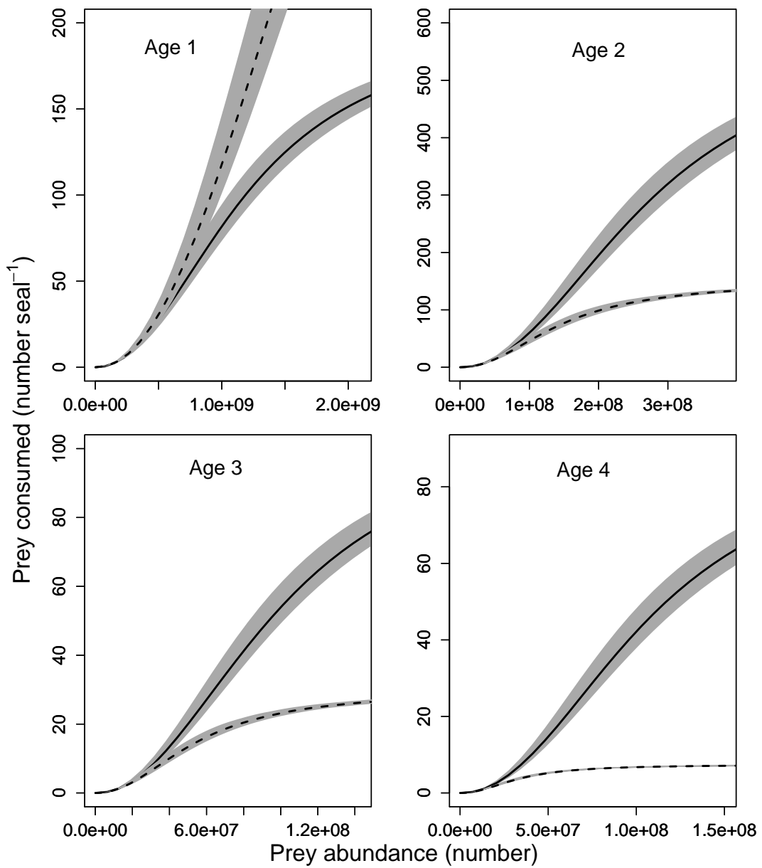
Figure 9: Predicted multi-age functional response of harp seal to cod for 2 distinct age-structures of the population. Solid line corresponds to the age-structure of the year 1984; dashed line corresponds to the age-structure of the year 1995 characterized by a high abundance of cod aged 1. Grey area represents 90% bootstrap confidence intervals. Scales were selected for readability along y -axes
