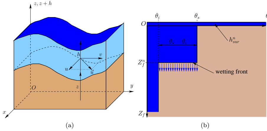
Figure 1: Illustration of (a) SW2D and (b) Green-Ampt models.
