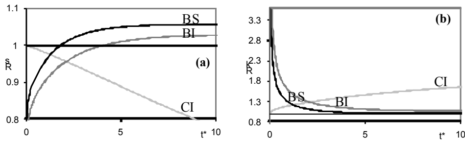
Figure 1. 1D infiltration data inverse modelling: ratios of estimated and target sorptivities -\hat{R}_S- (a) and saturated hydraulic conductivities -\hat{R}_K- (b) versus the scaled time ( t^* ).
