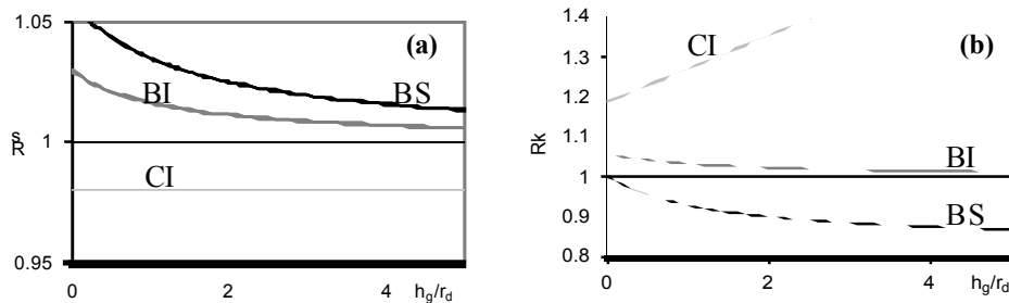
Figure 2. Ratios -\hat{R}_S- (a) and -\hat{R}_K- (b) versus the ratio of the scale parameter for water pressure ( h_g ) and the radius ( r_d ).
