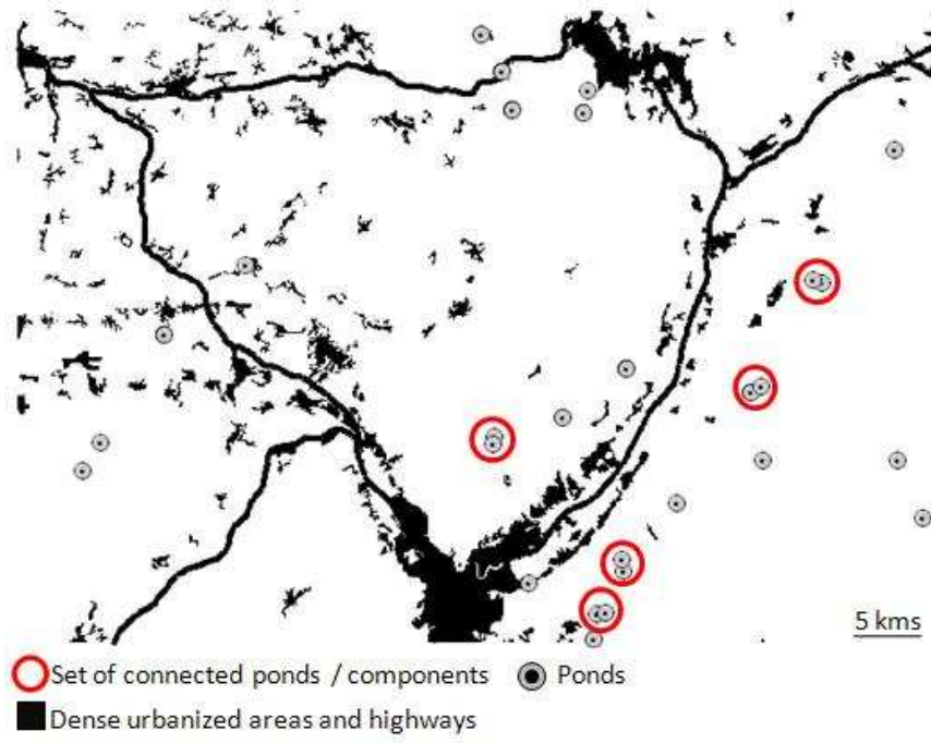
Figure 4. Set of connected ponds (components) identified with the computation of the Number of Components index (NC) using Conefor Sensinode software with a dispersal distance of 1500m (Nodes are not connected when PC equals 0 which correspond to a least cost path distance between nodes higher than 1500m).
