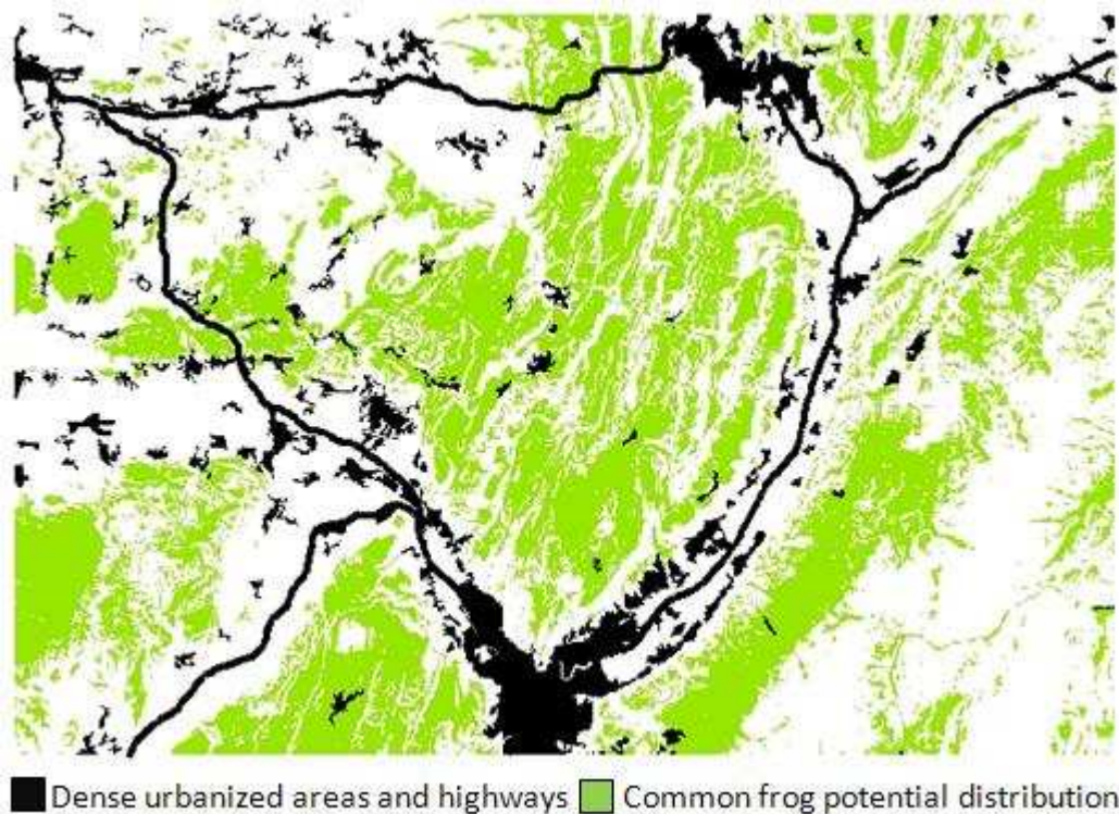
Figure 3. Potential distribution of the common frog (10 percentile training presence of 0.339 as the probability threshold) (area of 4067 km 2 ).
