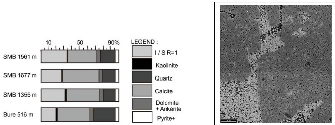
Figure 2: Example of analysis of two caprock faciès. Left: main mineral content of Callovo-Oxfordian argillites from the SMB and Bure area [xiv]. Right: SEM visualization of a dolomitic tight carbonate caprock, Comblanchien faciès [viii]. The thick black line indicates a scale of 50 \mu m.
