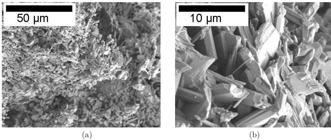
Figure 1: SEM image (secondary electron) of a plaster surface before bio-treatment (a) 1000 \times magnification, (b) 5000 \times magnification.
