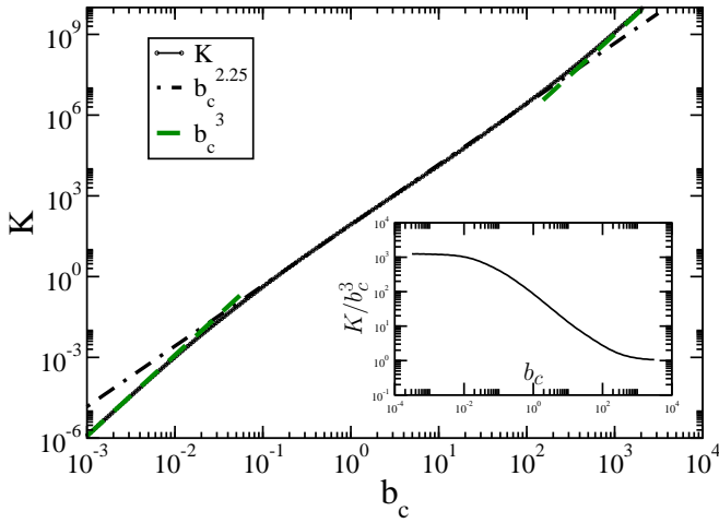
Figure 6: Permeability K as a function of b_c for 100 self-affine samples with H = 0.8 of size 1024 \times 1024 . The straight lines are b_c^{2.25} and b_c^3 respectively.
