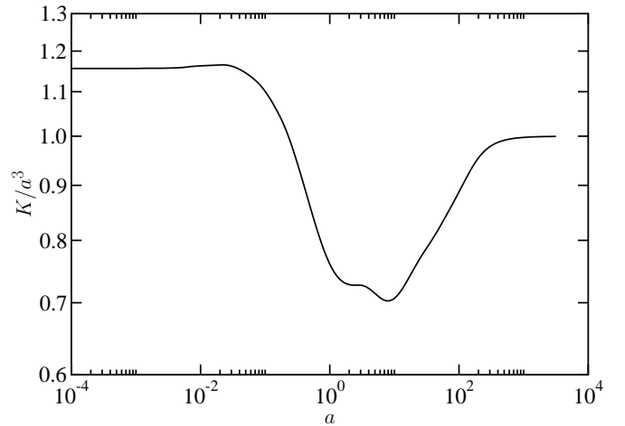
Figure 5: Permeability K/a^3 as a function of opening a for 100 self-affine samples of size 1024. For small and large a , K \sim a^3 , but with different prefactors.
