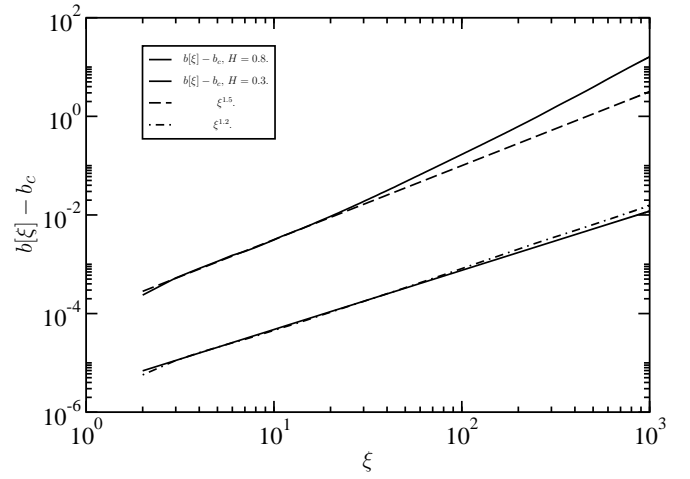
Figure 7: Ordered sequences b[\xi] - b_c from 1000 samples of size 1024 \times 1024 with Hurst exponents H = 0.8 and H = 0.3 respectively. The straight lines are proportional to \xi^{1.5} and \xi^{1.2} respectively.
