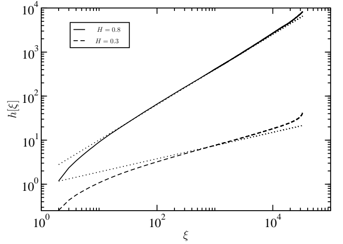
Figure 3: Ordered and averaged sequence \bar{h}[\xi] based on 1000 self-affine h(x) with Hurst exponents equal to 0.8 and 0.3 respectively. The data consists of 1000 samples of length 2^{15} . The straight lines are \xi^{0.8} and \xi^{0.3} respectively.
