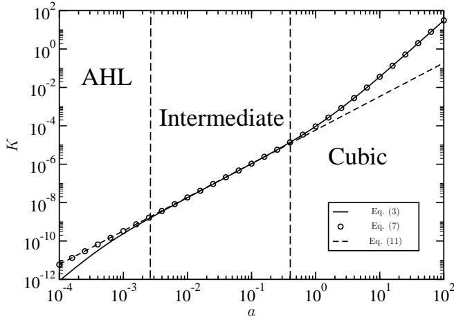
Figure 2: Permeability K averaged over 1000 fields of length 2^{15} with h distributed according to a power law p(h) \sim h^{\alpha-1} on the unit interval, where \alpha = 1.25 . Solid line and open circles show respectively the permeability K calculated from Eqs. (3) and (7) respectively as a function of minimum opening a . The three scaling regimes are delimited by vertical lines. The dashed line represent a^{3-\alpha} = a^{1.75} .
