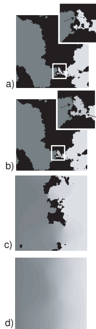
Figure 8: Pressure field in gray levels a self-affine realization. The flow is from left to right. Dark regions correspond to contact zones. From top to bottom: ((b - b_c) = 10^{-4} (“AHL” regime, the arrow indicates the percolation point), 0.5 (cross over regime, the arrows show the two significant pressure drop corresponding to the two major barriers), 28 (cross over regime) and 97 (cubic law regime).
