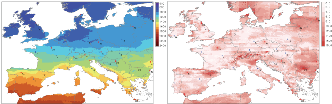
Fig. 1: Yearly sum of global horizontal irradiation, average of all five data bases [kWh/m 2 ] (left), uncertainty at 95% confidence interval from the comparison of the five data bases. [%] (right).
