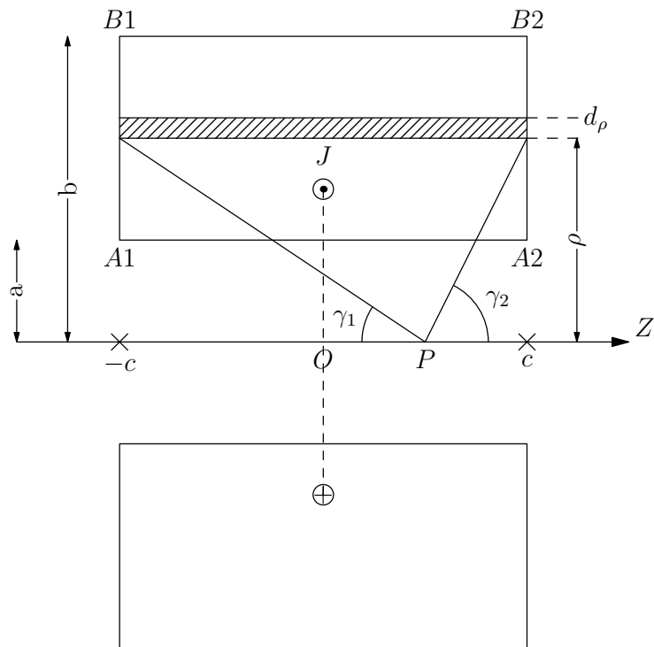
Figure 8: Thick coil cross-section illustrating the magnetic induction generated along the z -axis. a and b are the inner- and outer-radius of the coil of section S ( A_1 - B_1 - B_2 - A_2 ), respectively, c is the half-length.
