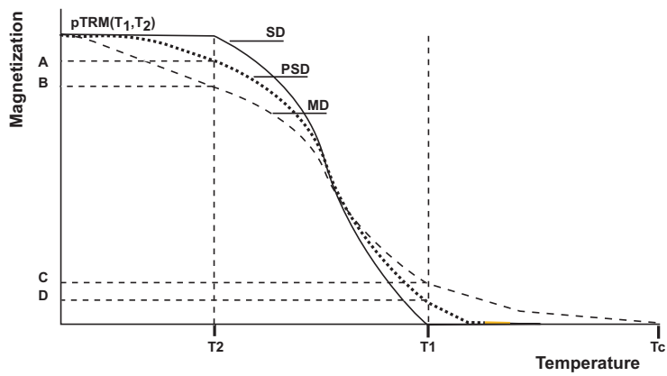
Figure 6: pTRM tail-check: Continuous thermal demagnetization of pTRM( T_1, T_2 ) illustrating two different pTRM-tails. The low-temperature pTRM-tail corresponds to the part of pTRM( T_1, T_2 ) removed at T_2 . The high-temperature pTRM-tail corresponds to the part of pTRM( T_1, T_2 ) unrecovered at T_1 . A(B) is the low-temperature pTRM-Tail measured at room temperature for PSD(MD) grains. C(D) is the high-temperature pTRM-Tail measured at room temperature for PSD (MD) grains. Figure redrawn from Plenier et al [18].
