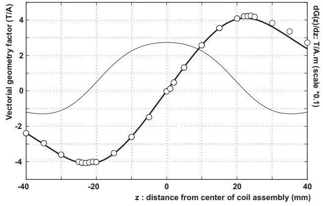
Figure 2: Vectorial geometry factor profile G(z) . The calculate profile (bold curve) is compared to the experimental measures (open circles). The thin solid line is the calculated derivative dG(z)/dz . z=0 corresponds to the center of the coil assembly.
