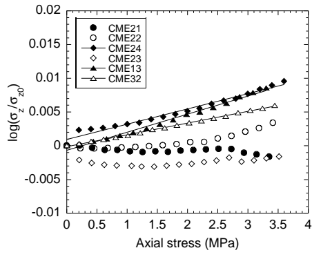
Figure 8. Logarithm of the rock conductivity versus axial stress for the six studied samples.
