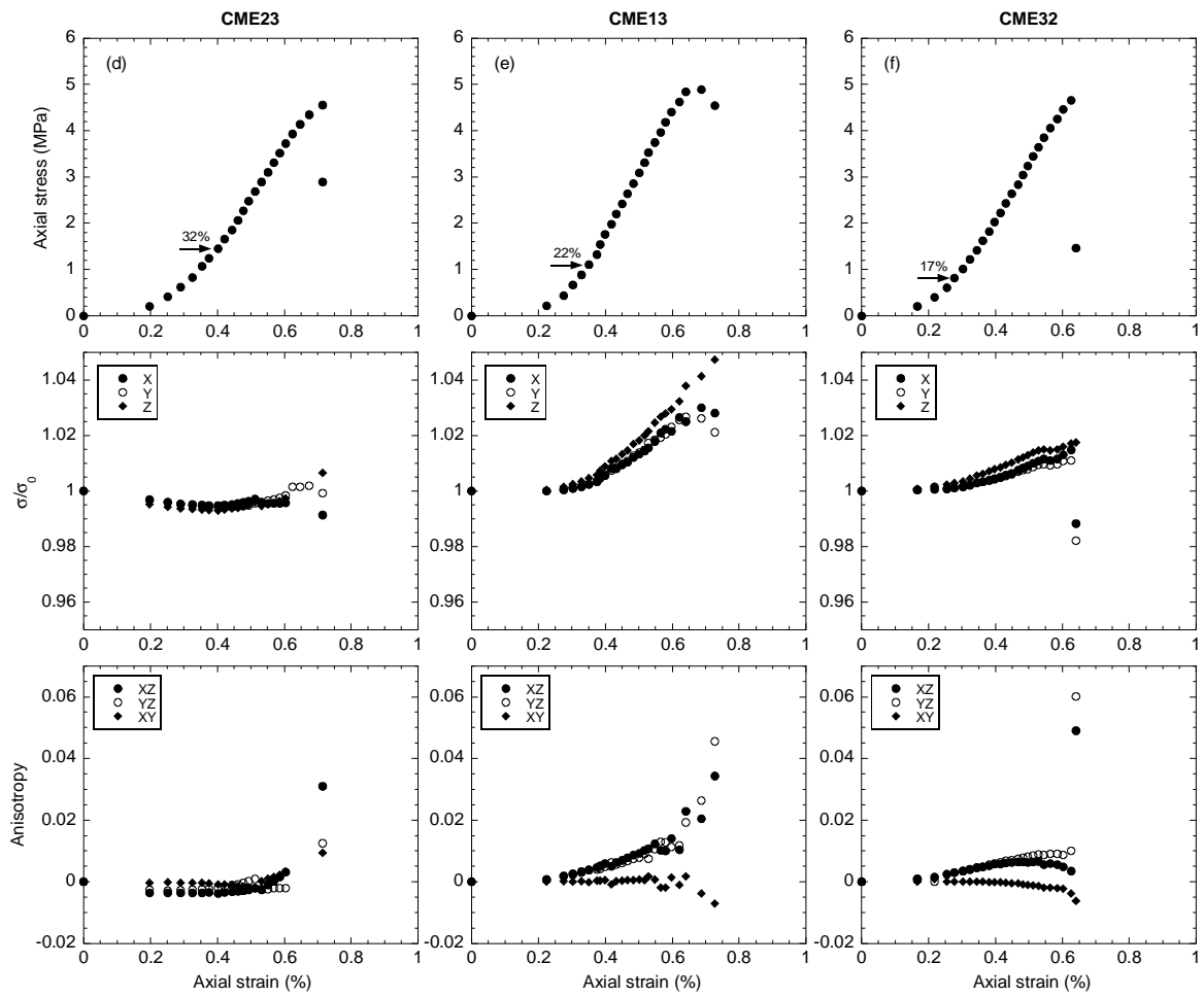
Figure 4. Axial stress, rock conductivity, and electrical anisotropy, versus axial strain. 4a: CME21 sample; 4b: CME22 sample; 4c: CME24 sample; 4d: CME23 sample; 4e: CME13 sample; 4f: CME32 sample.
