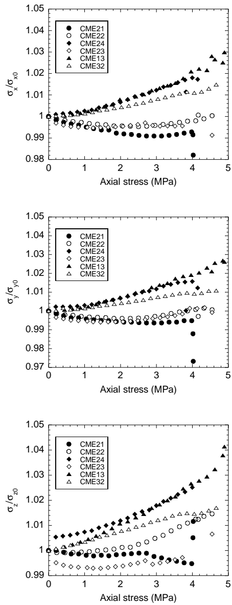
Figure 6. Rock conductivity versus axial stress for the six studied samples.
