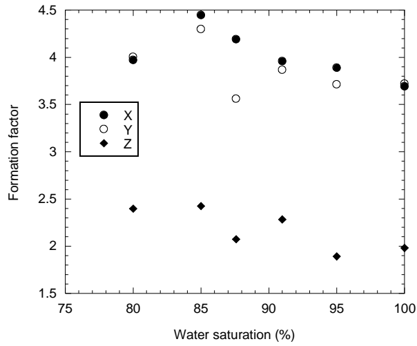
Figure 3. Initial formation factor in the three directions X , Y , Z versus water saturation of the samples.
